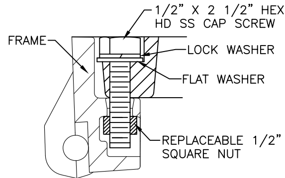
BOLT DETAIL
